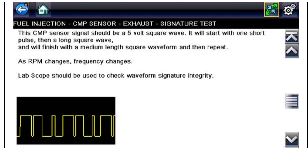
Figure 4-14 Waveform Example
